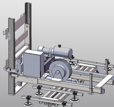
Forklift Attachments
