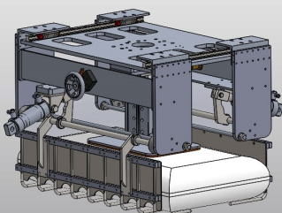
Bag Grippers Custom EOAT
