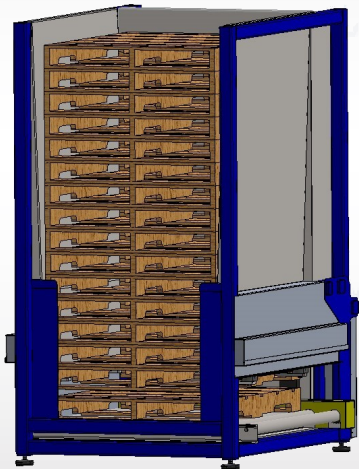
Pallet Dispensers
